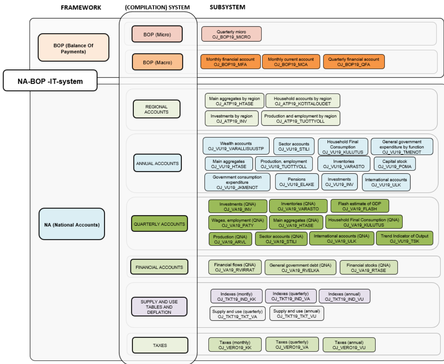
Figure 3: IT-system structure
